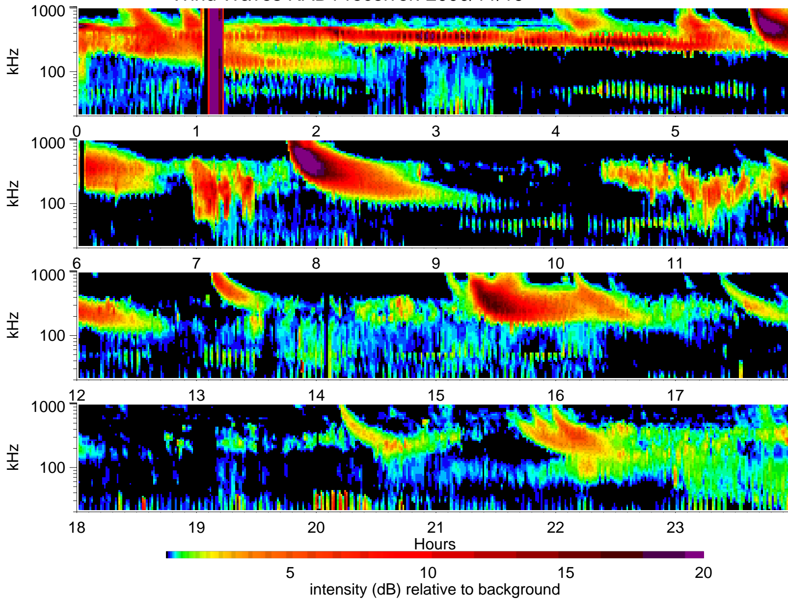
Wind Waves RAD1 receiver: 2000/11/19
