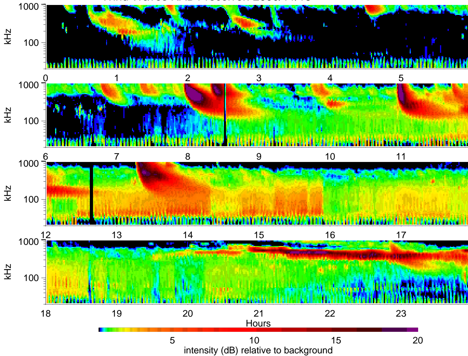
Wind Waves RAD1 receiver: 2000/11/18
