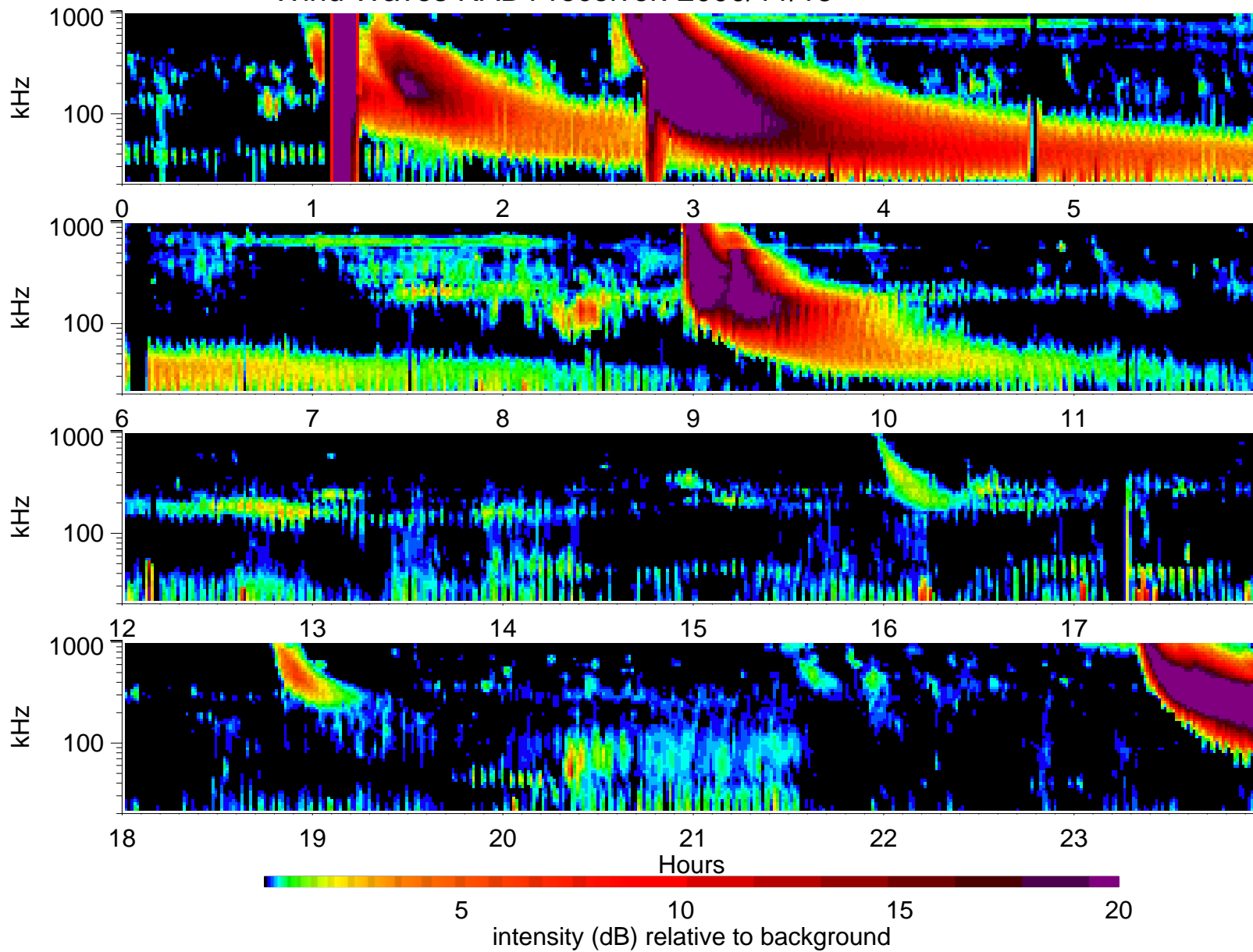
Wind Waves RAD1 receiver: 2000/11/15
