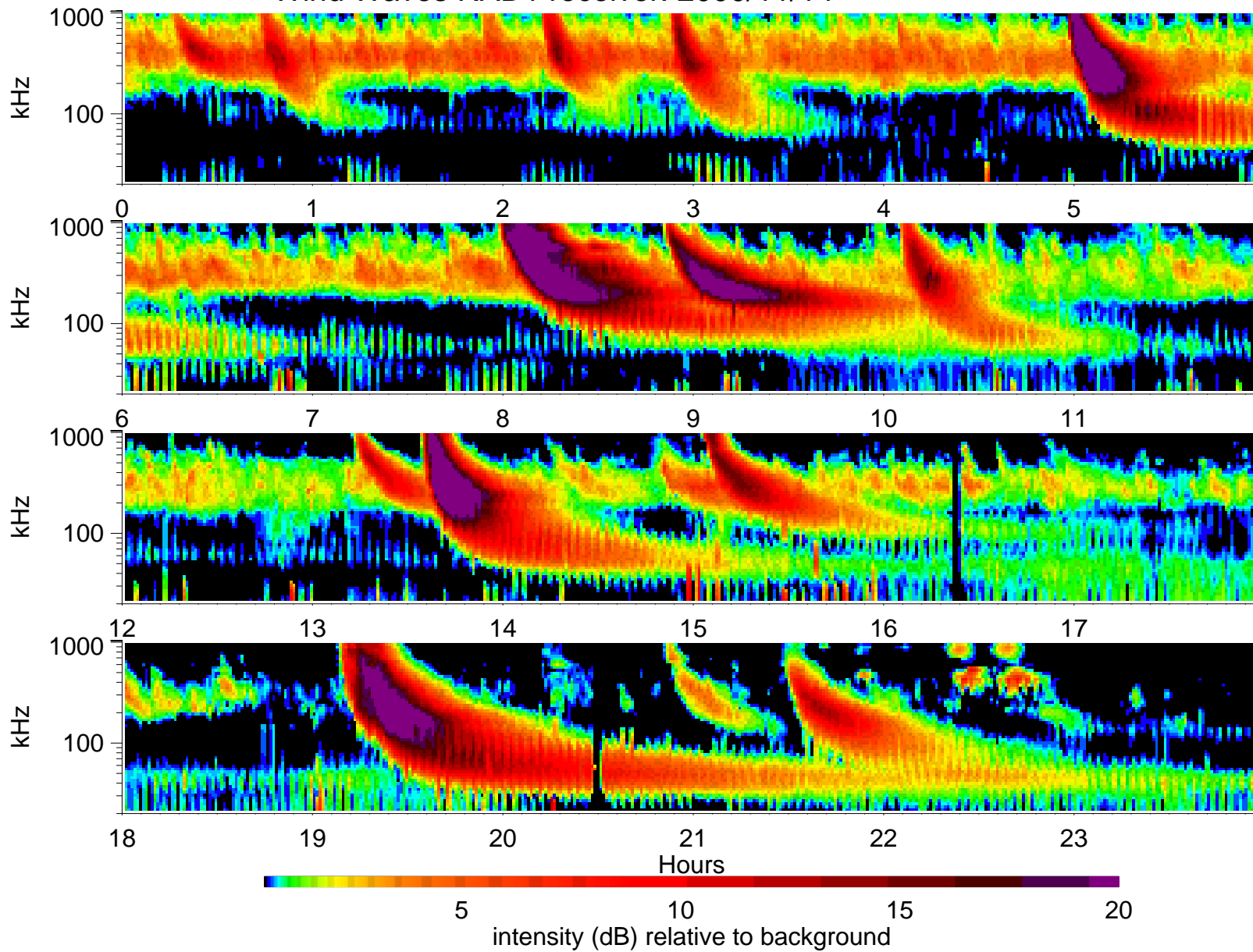
Wind Waves RAD1 receiver: 2000/11/14
