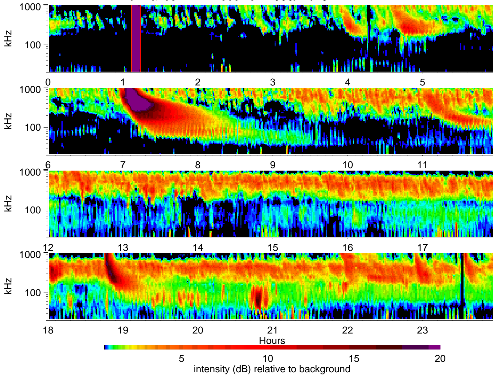
Wind Waves RAD1 receiver: 2000/11/13
