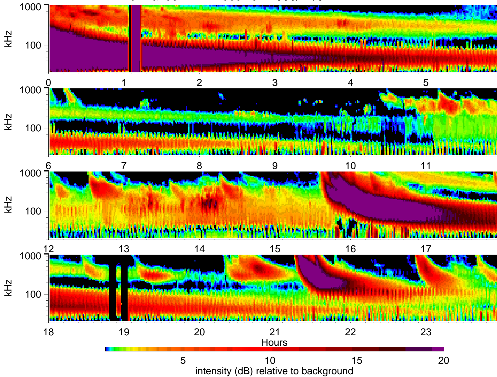
Wind Waves RAD1 receiver: 2000/11/9
