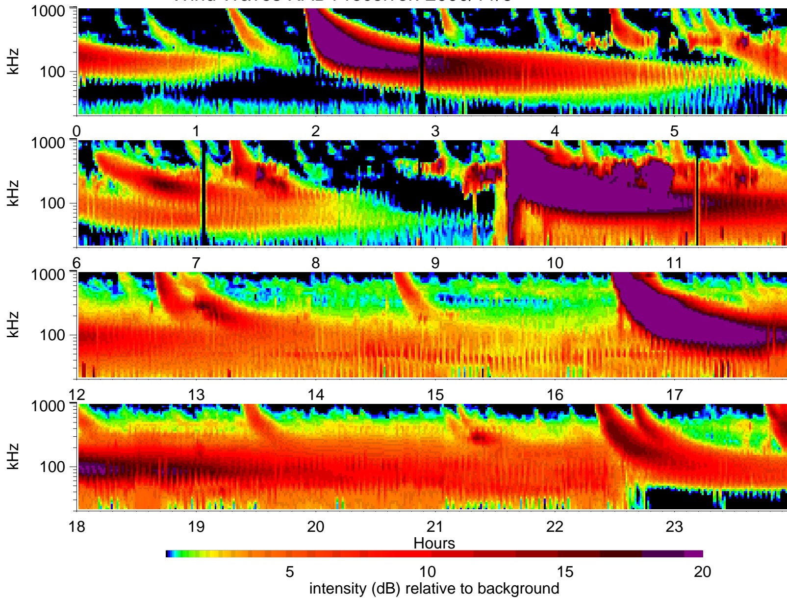
Wind Waves RAD1 receiver: 2000/11/6
