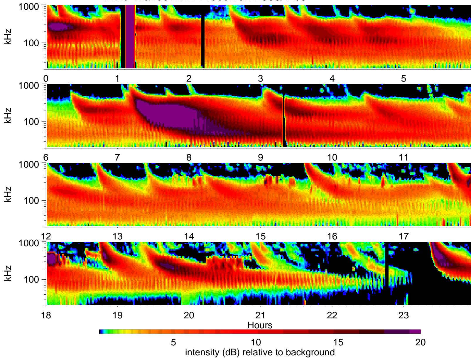
Wind Waves RAD1 receiver: 2000/11/5
