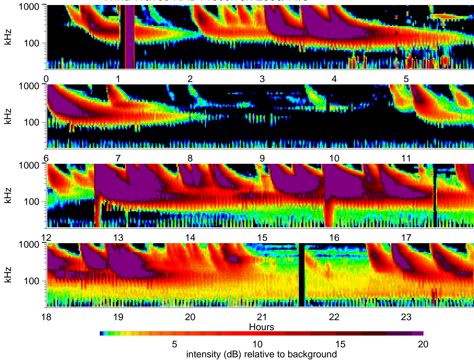
Wind Waves RAD1 receiver: 2000/11/3
