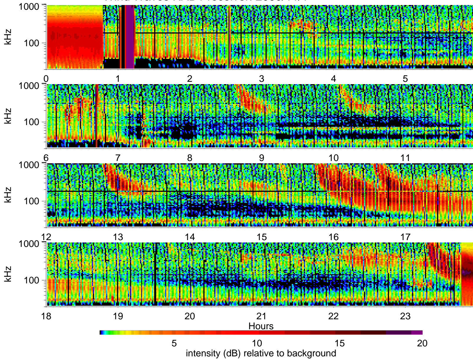
Wind Waves RAD1 receiver: 2000/11/1
