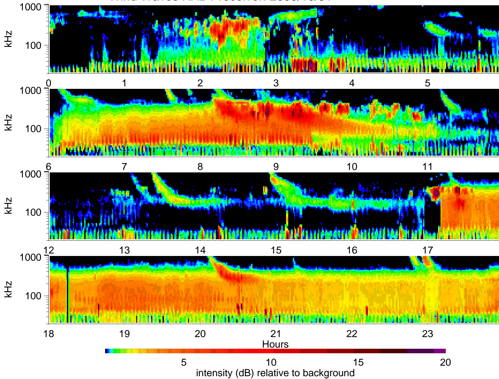
Wind Waves RAD1 receiver: 2000/10/31
