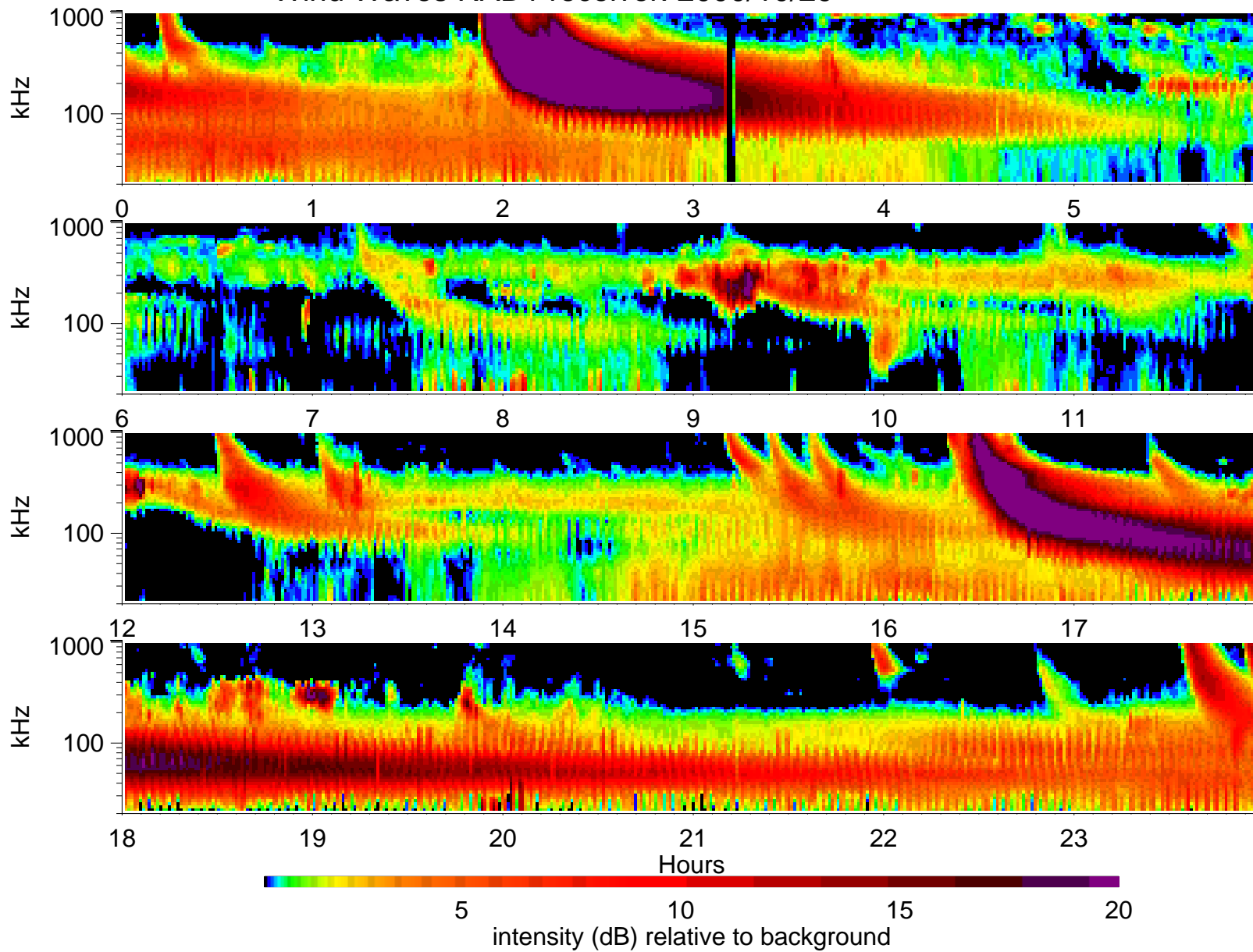
Wind Waves RAD1 receiver: 2000/10/29
