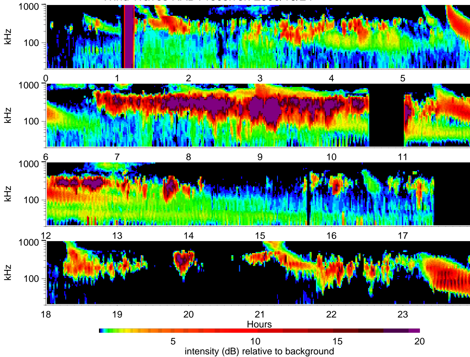
Wind Waves RAD1 receiver: 2000/10/24
