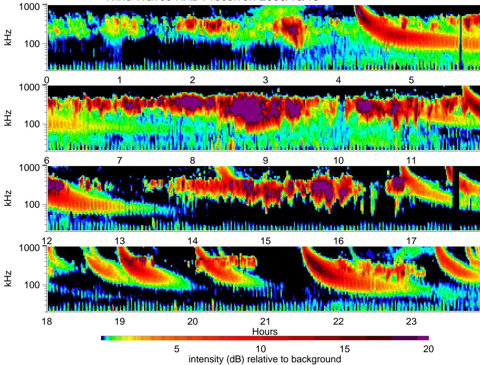
Wind Waves RAD1 receiver: 2000/10/19
