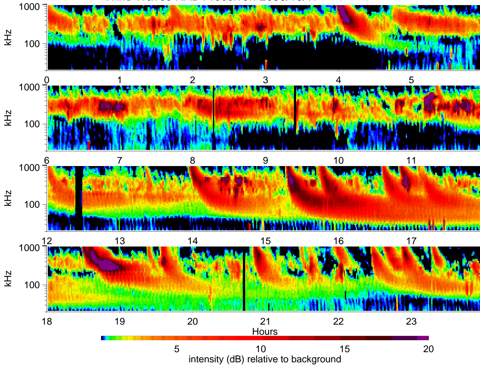
Wind Waves RAD1 receiver: 2000/10/17
