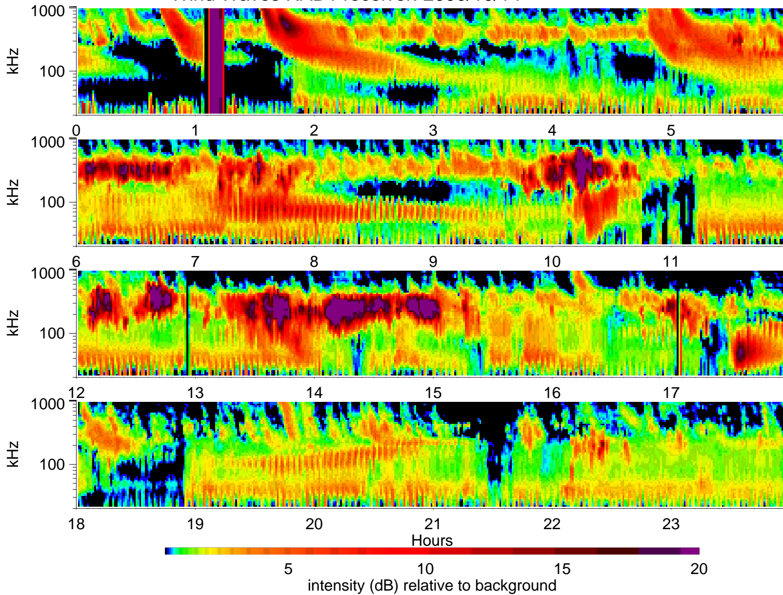
Wind Waves RAD1 receiver: 2000/10/14
