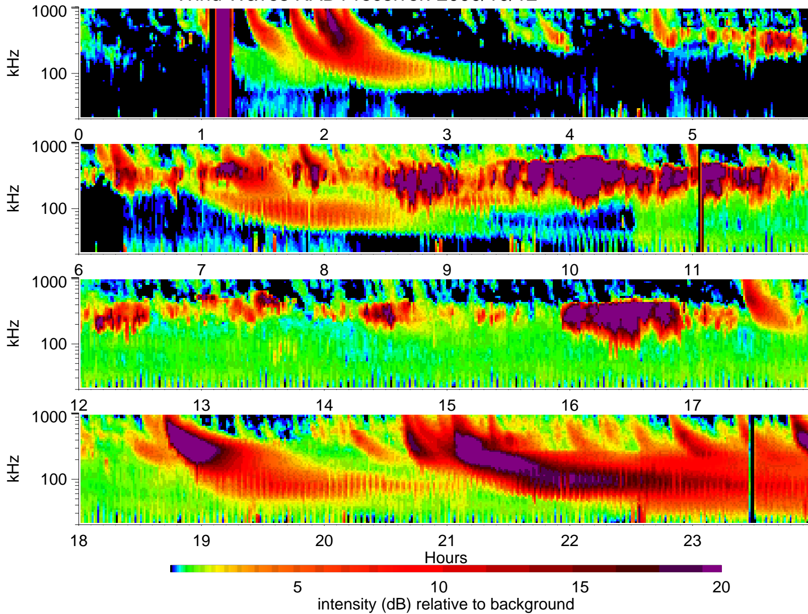
Wind Waves RAD1 receiver: 2000/10/12
