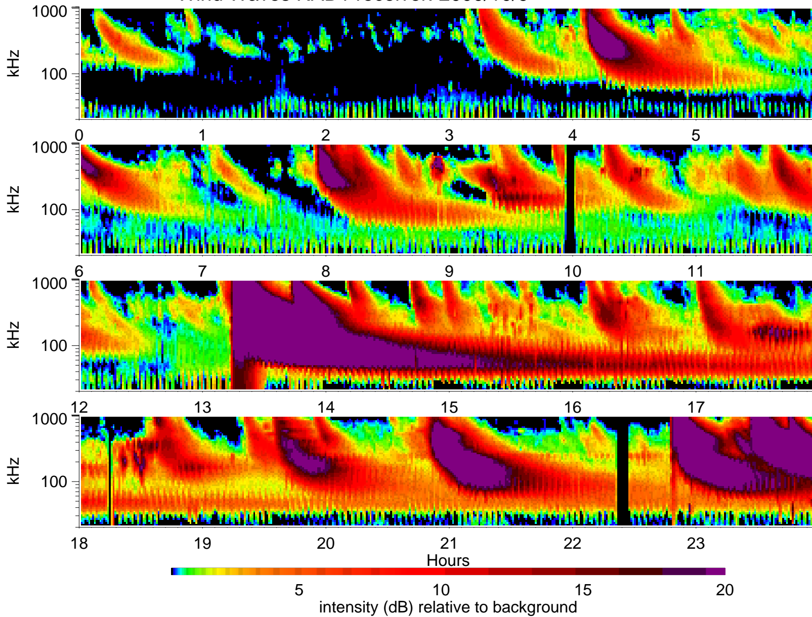
Wind Waves RAD1 receiver: 2000/10/9
