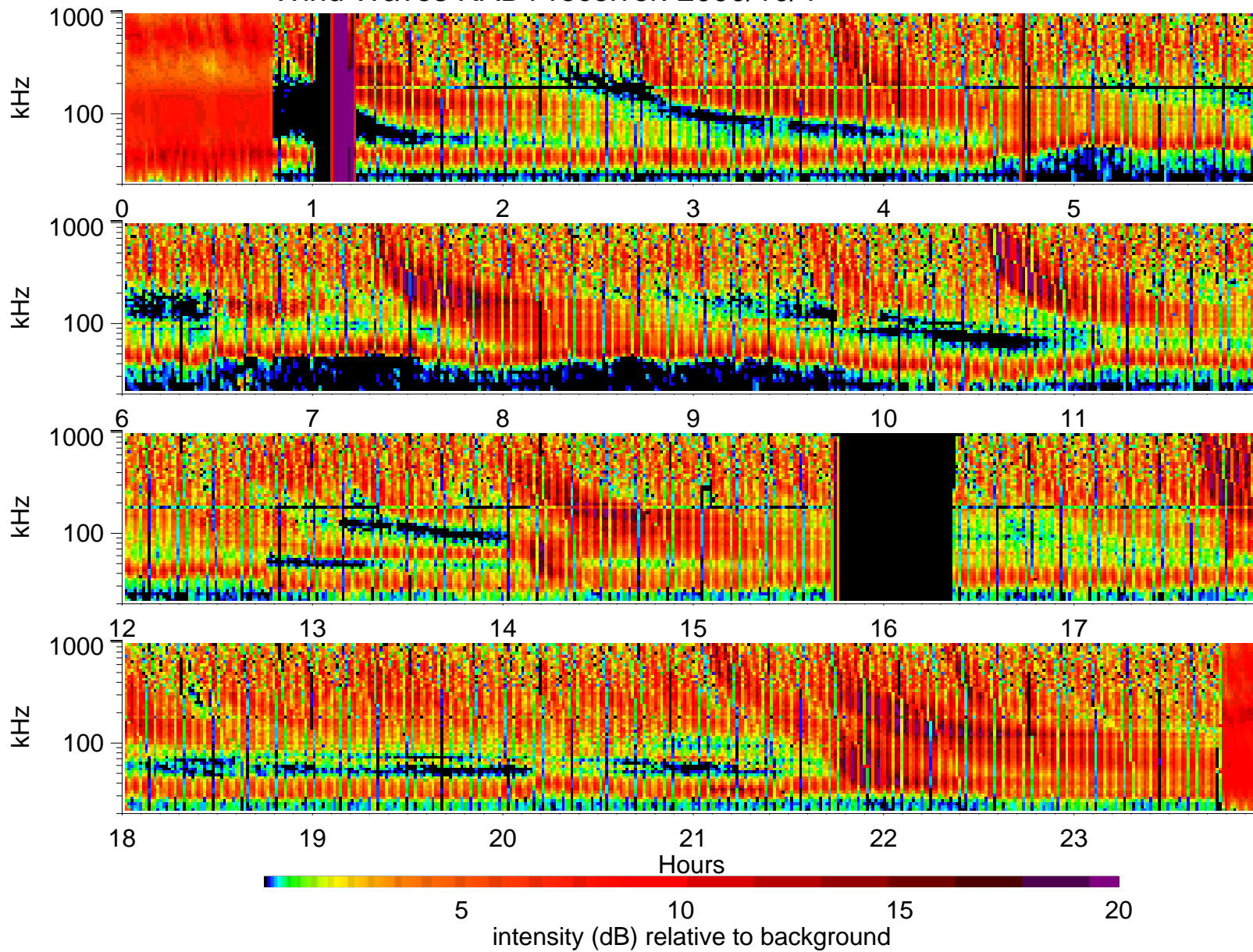
Wind Waves RAD1 receiver: 2000/10/4
