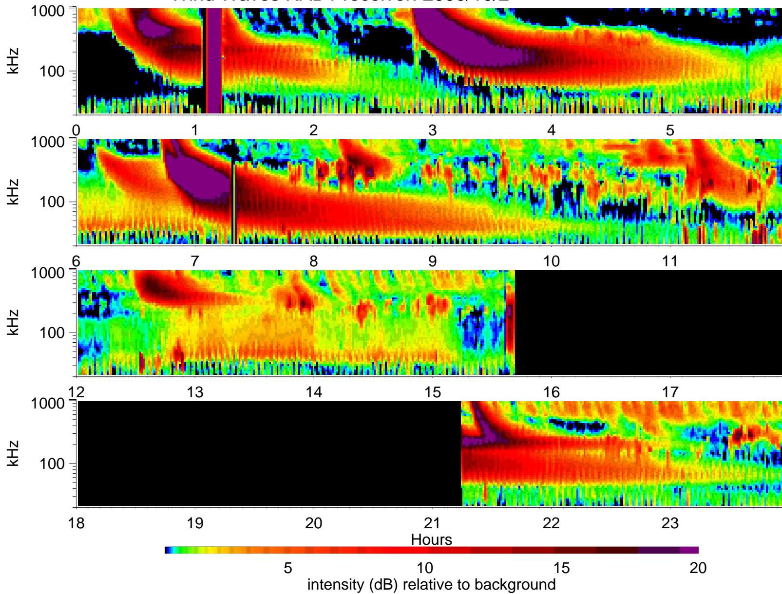
Wind Waves RAD1 receiver: 2000/10/2
