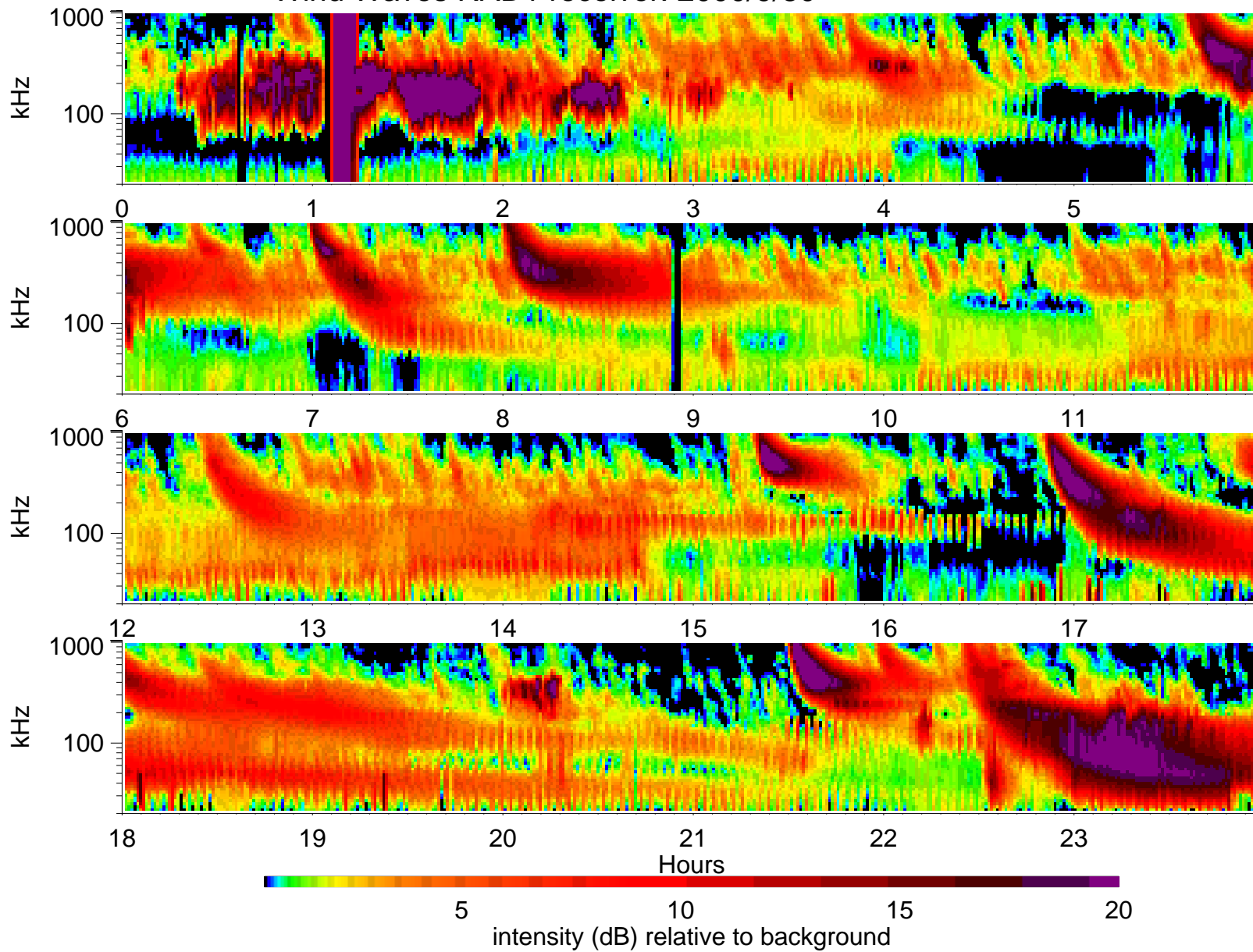
Wind Waves RAD1 receiver: 2000/9/30
