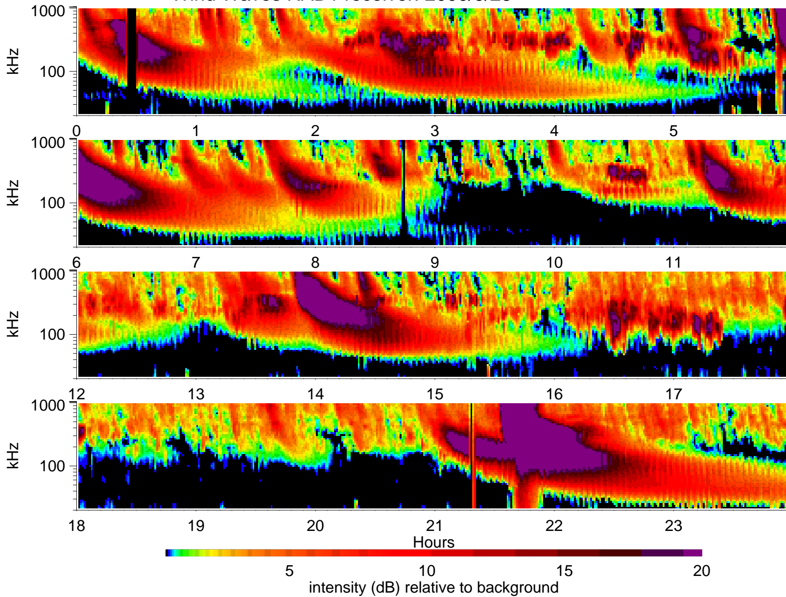
Wind Waves RAD1 receiver: 2000/9/23
