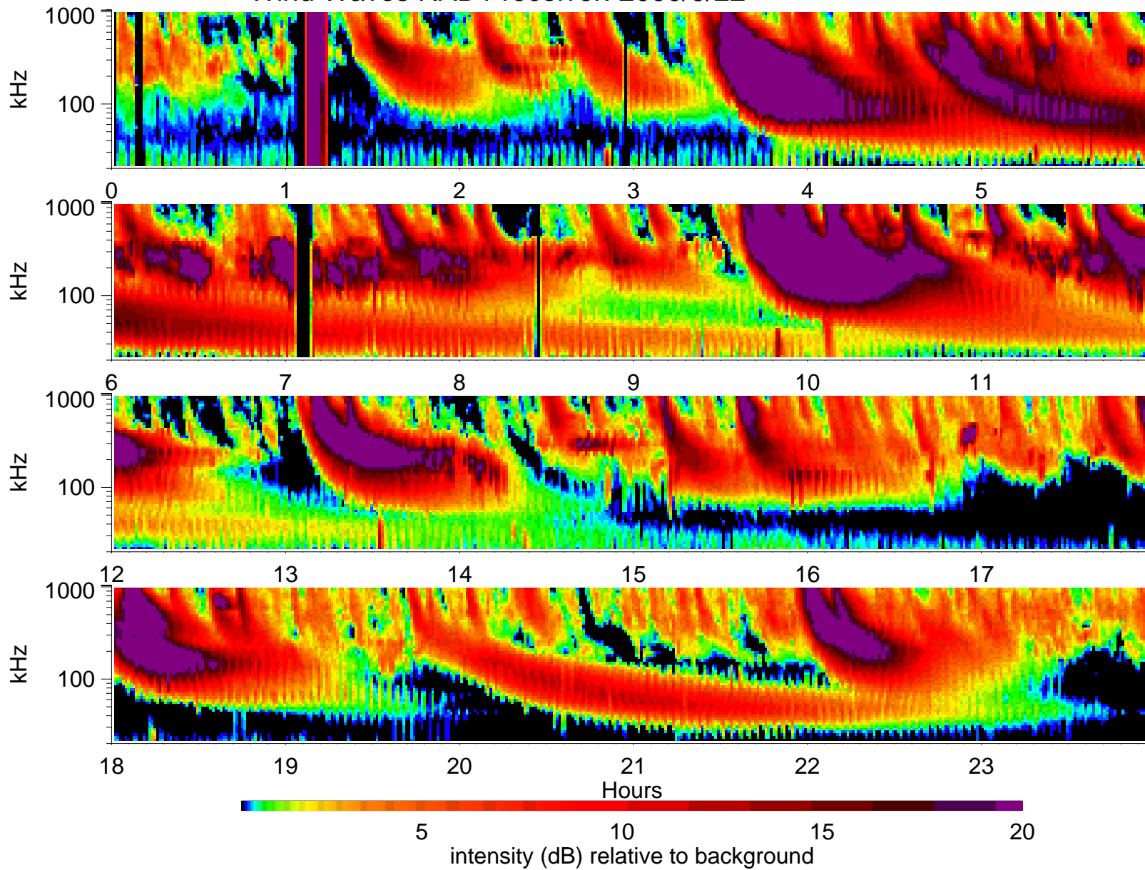
Wind Waves RAD1 receiver: 2000/9/22
