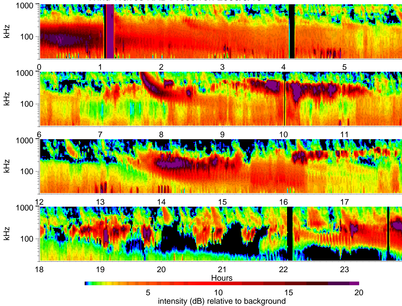
Wind Waves RAD1 receiver: 2000/9/18
