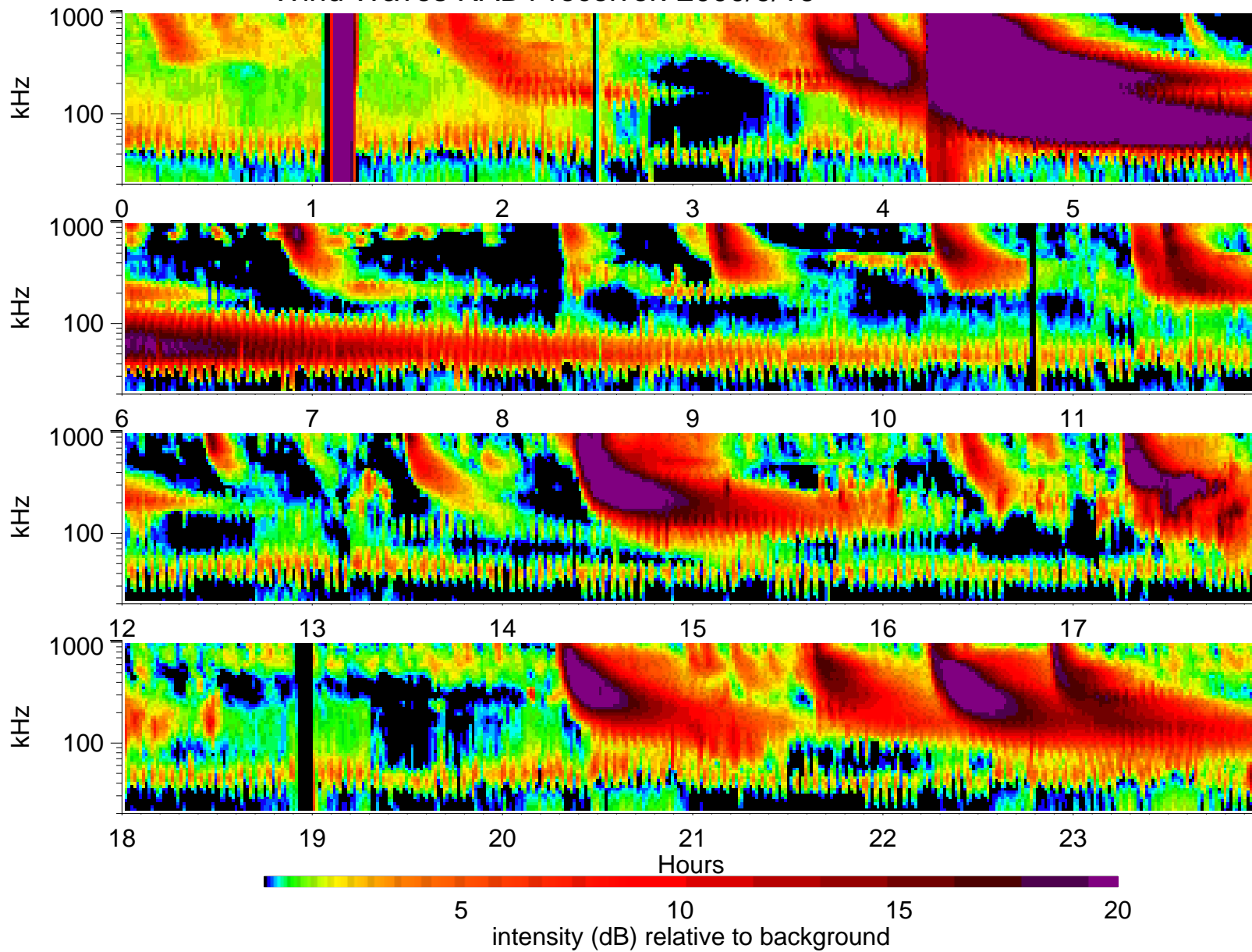
Wind Waves RAD1 receiver: 2000/9/16
