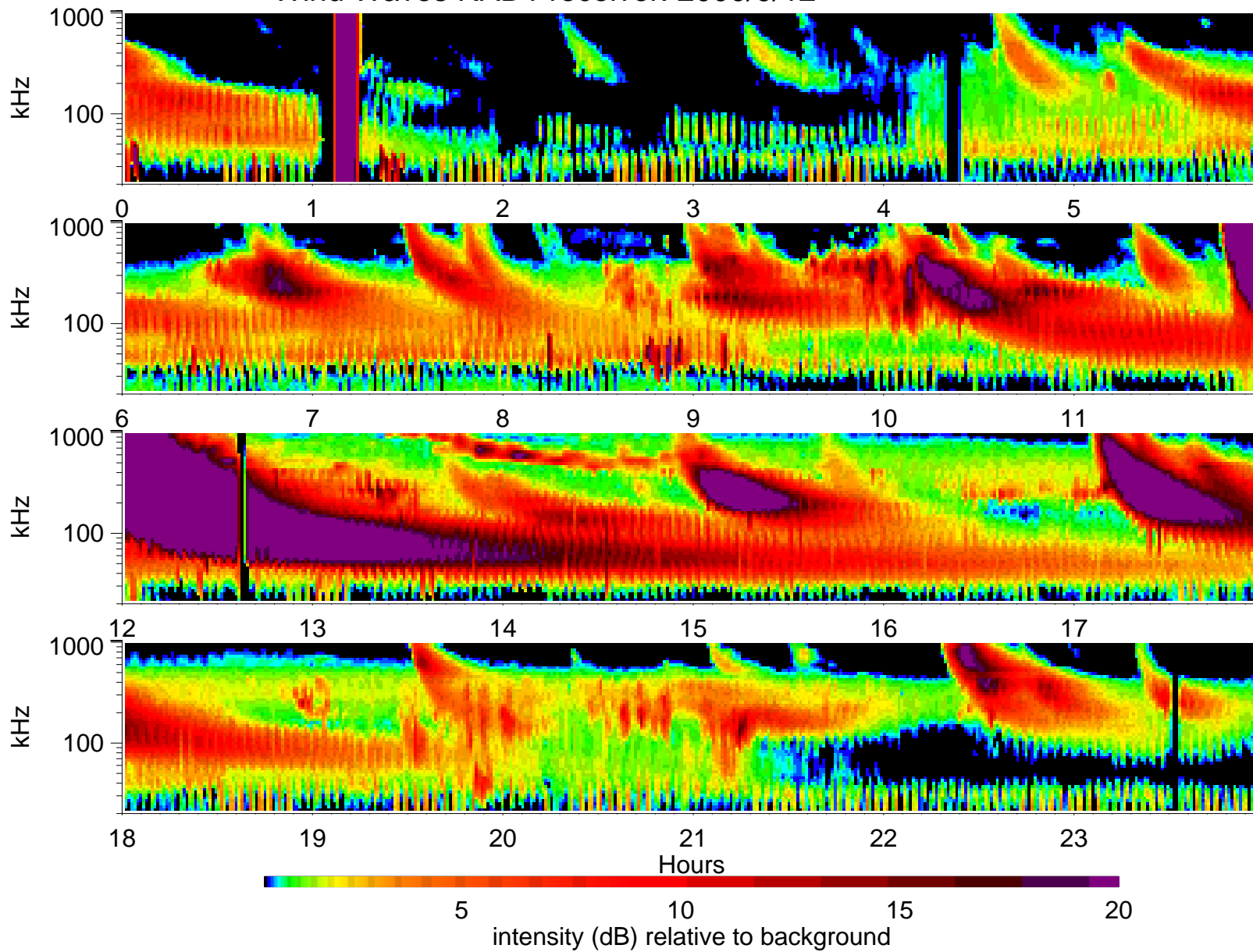
Wind Waves RAD1 receiver: 2000/9/12
