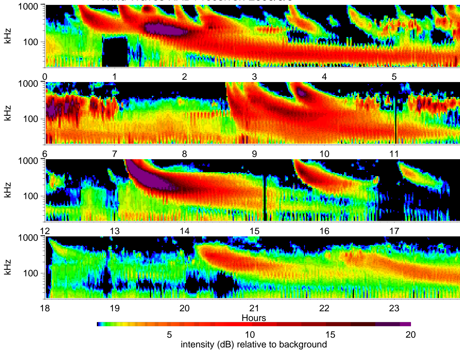
Wind Waves RAD1 receiver: 2000/9/9
