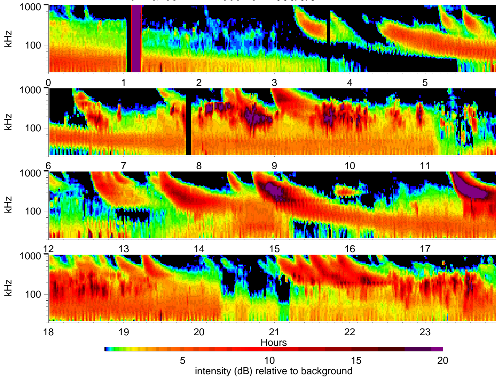
Wind Waves RAD1 receiver: 2000/9/8
