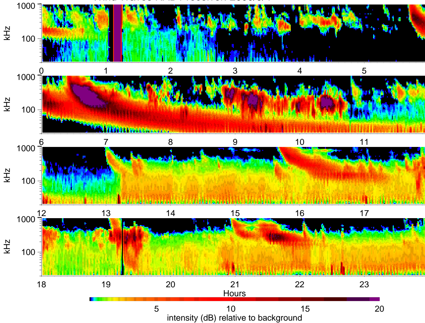
Wind Waves RAD1 receiver: 2000/9/4
