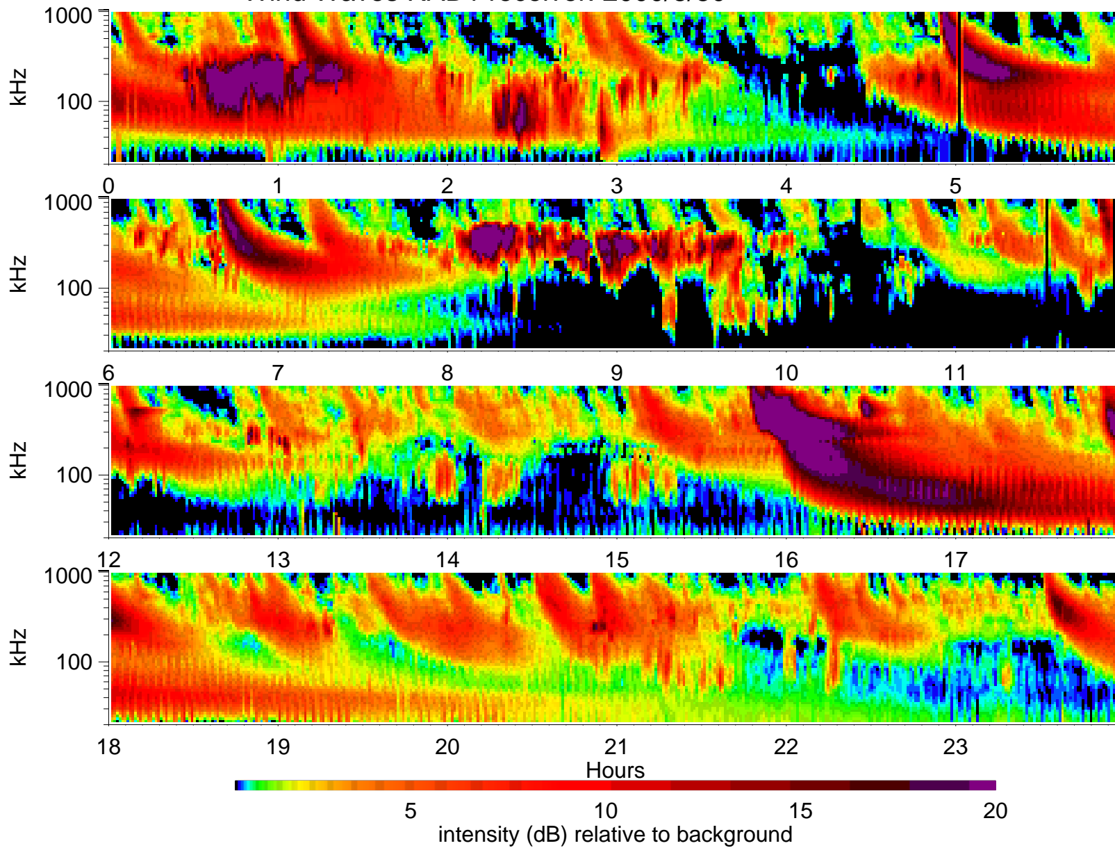
Wind Waves RAD1 receiver: 2000/8/30
