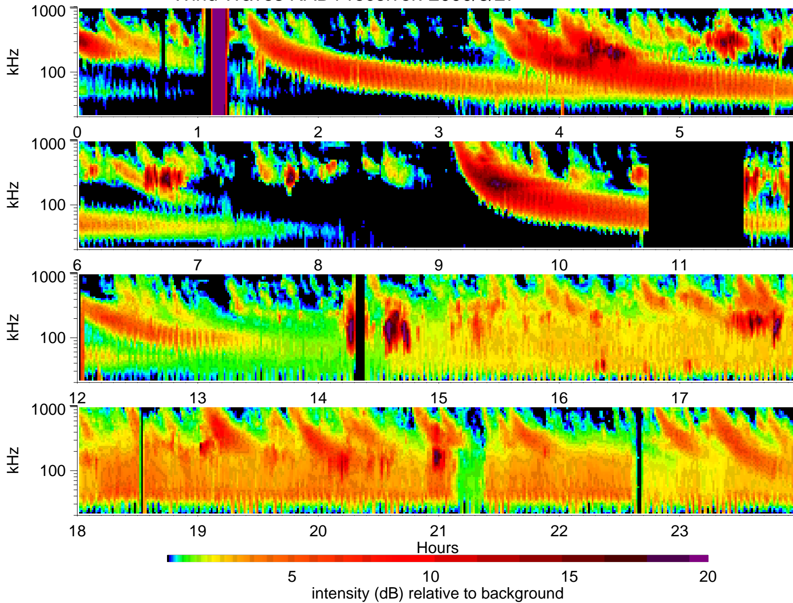
Wind Waves RAD1 receiver: 2000/8/27
