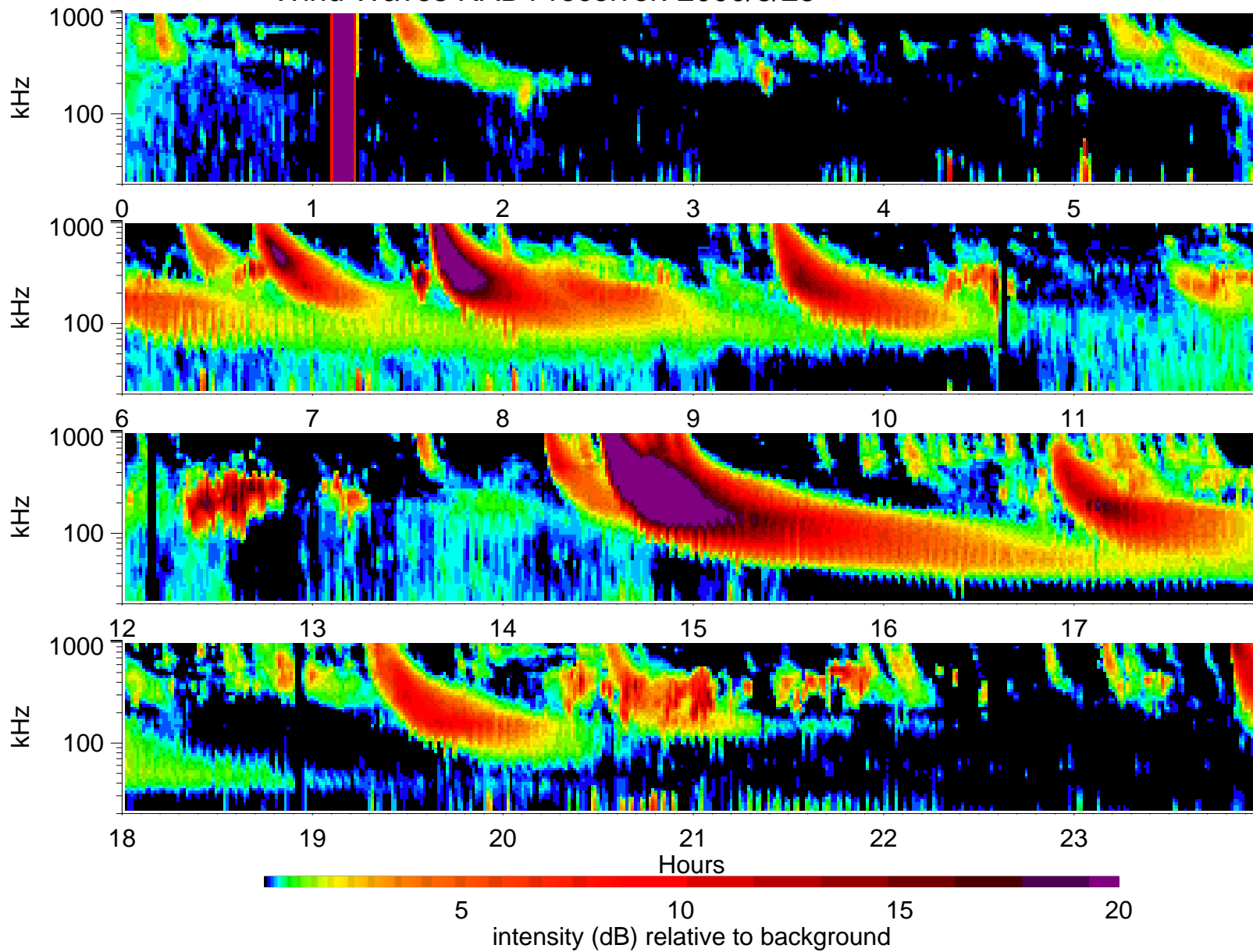
Wind Waves RAD1 receiver: 2000/8/25
