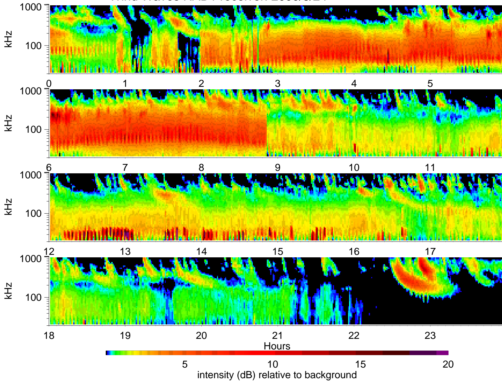
Wind Waves RAD1 receiver: 2000/8/24
