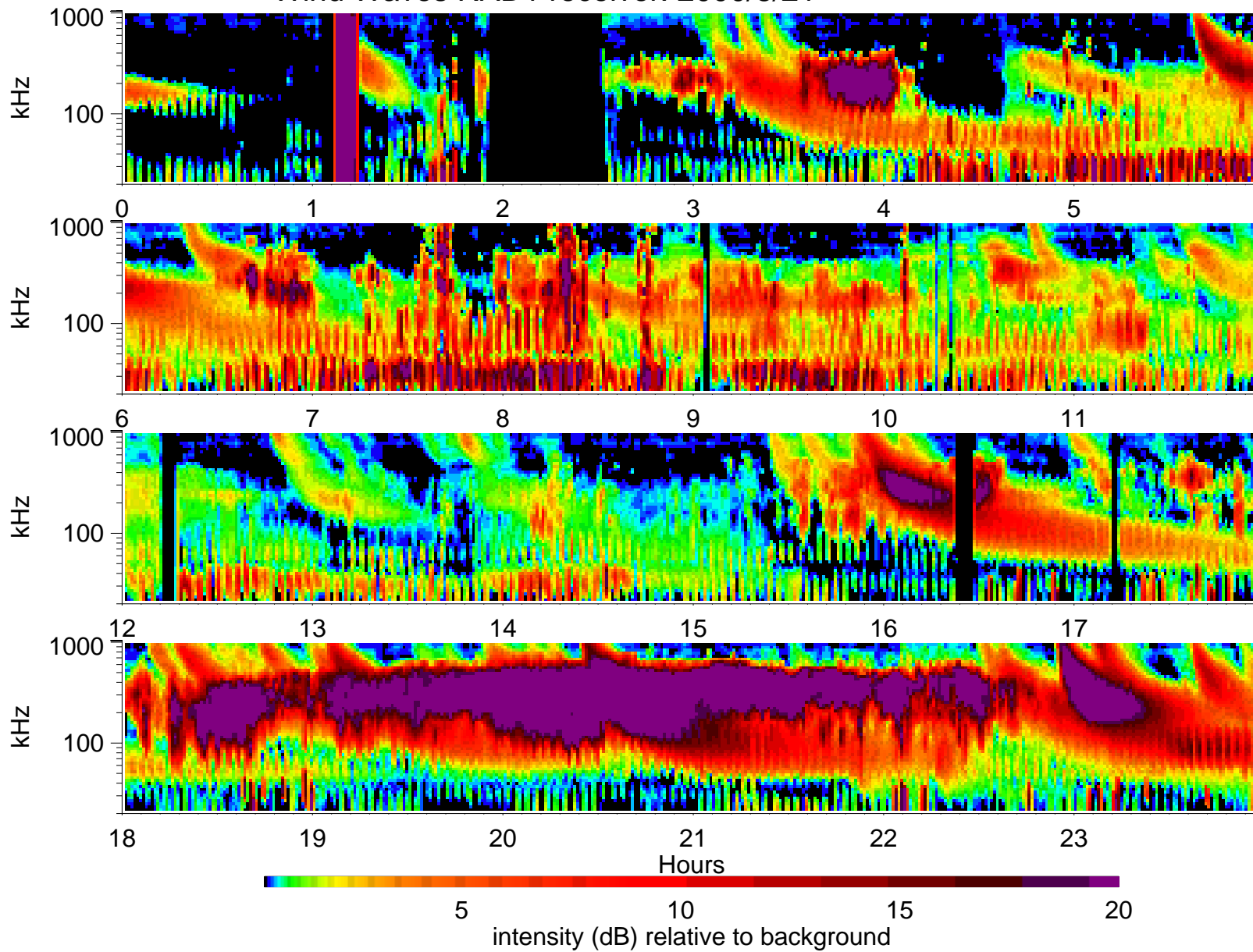
Wind Waves RAD1 receiver: 2000/8/21
