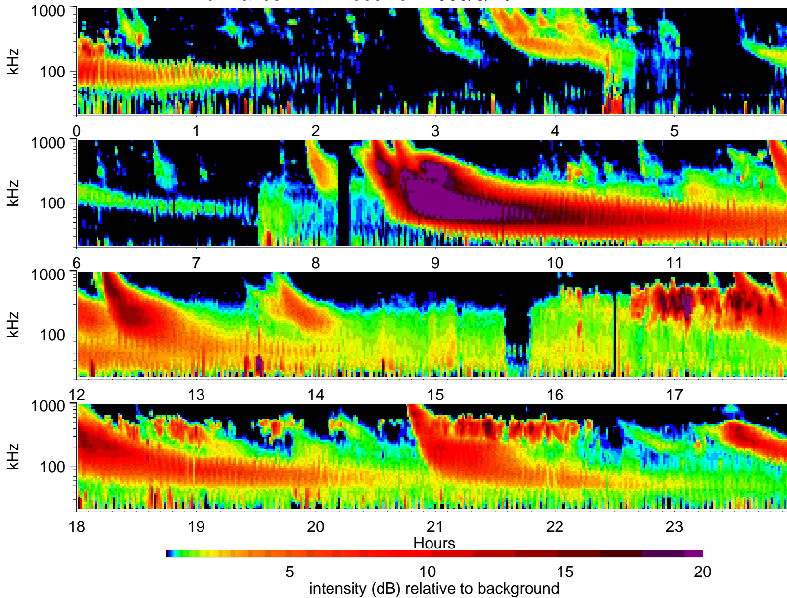
Wind Waves RAD1 receiver: 2000/8/20
