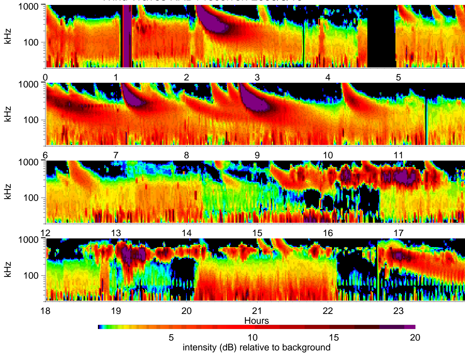
Wind Waves RAD1 receiver: 2000/8/19
