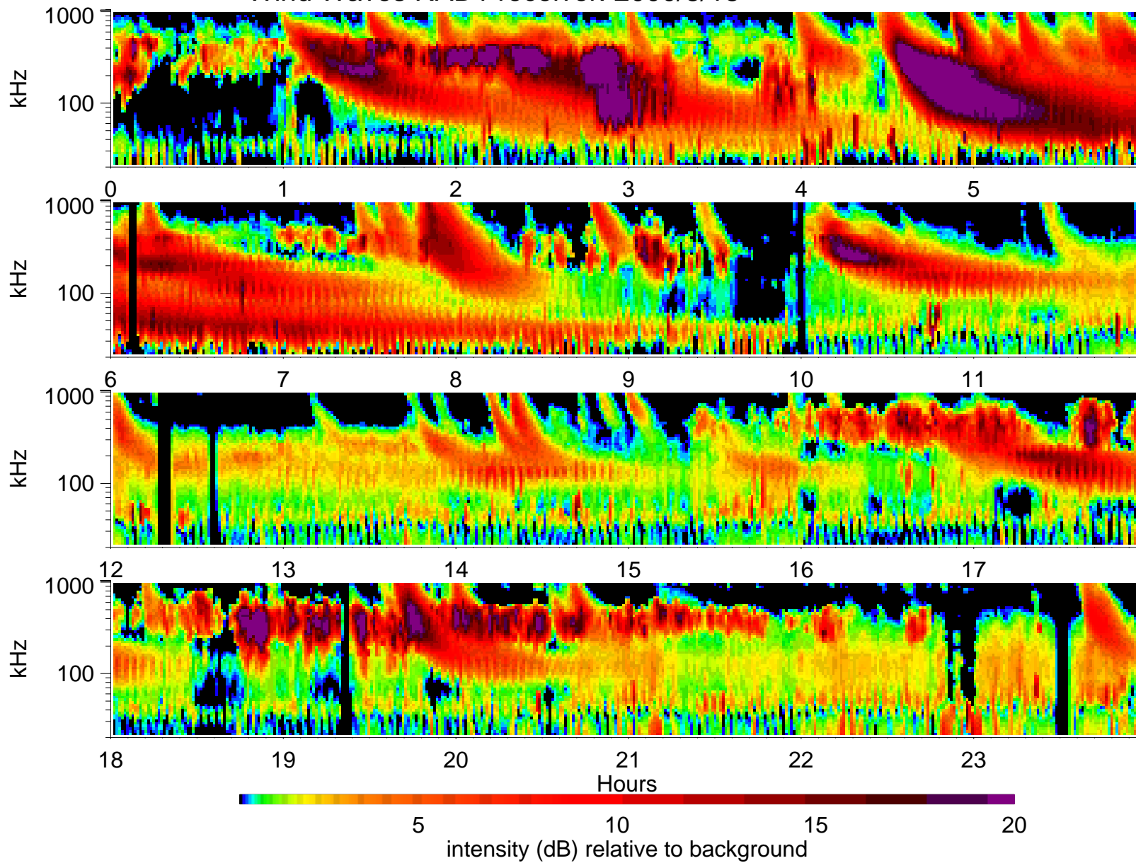
Wind Waves RAD1 receiver: 2000/8/18
