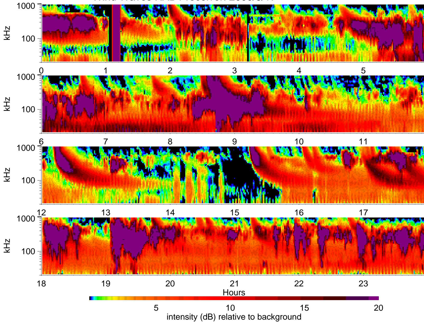
Wind Waves RAD1 receiver: 2000/8/17
