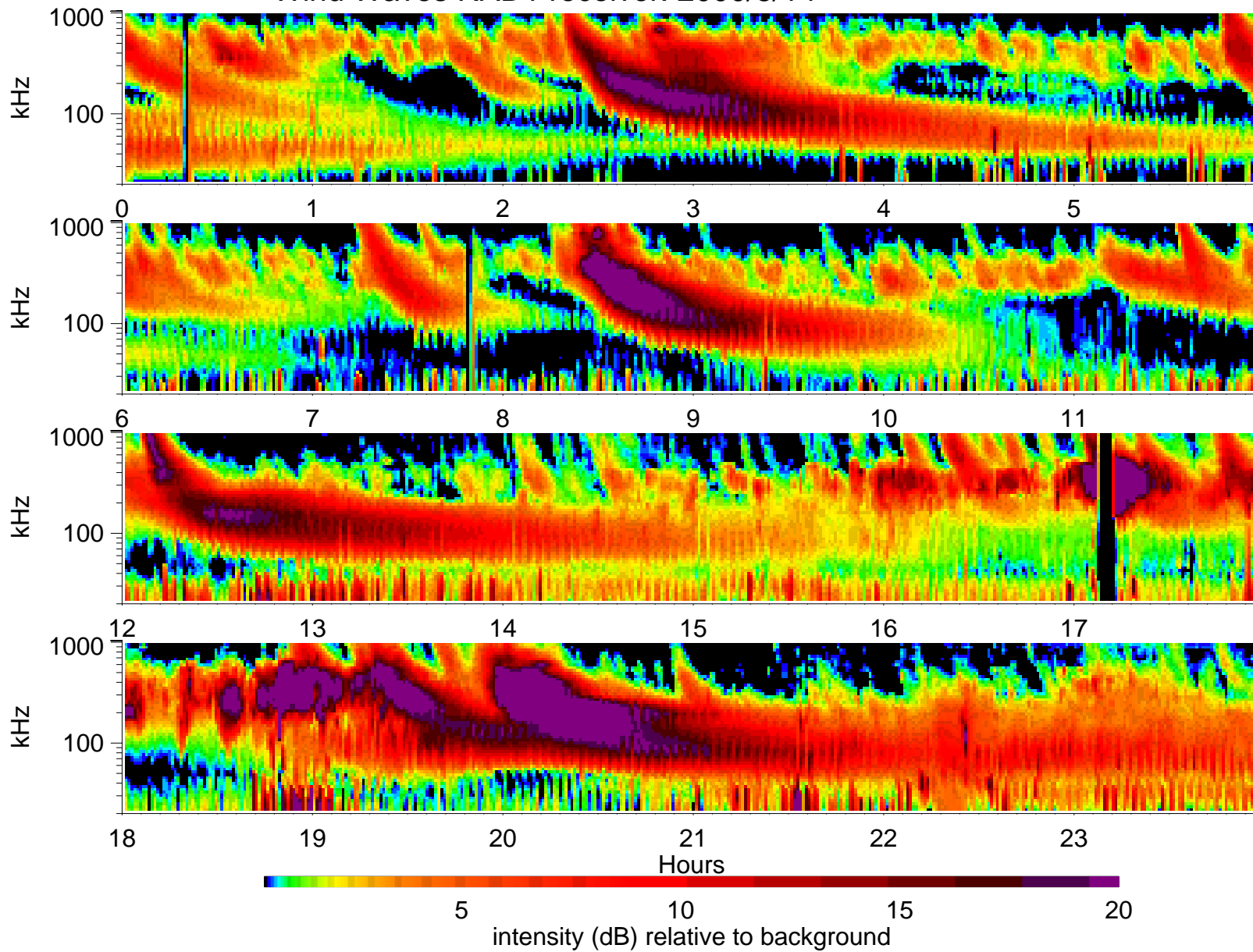
Wind Waves RAD1 receiver: 2000/8/14
