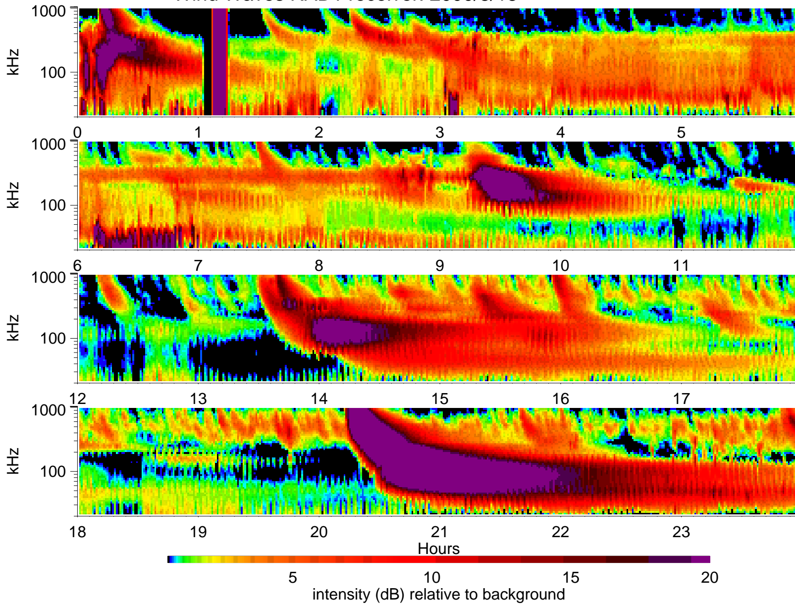
Wind Waves RAD1 receiver: 2000/8/13
