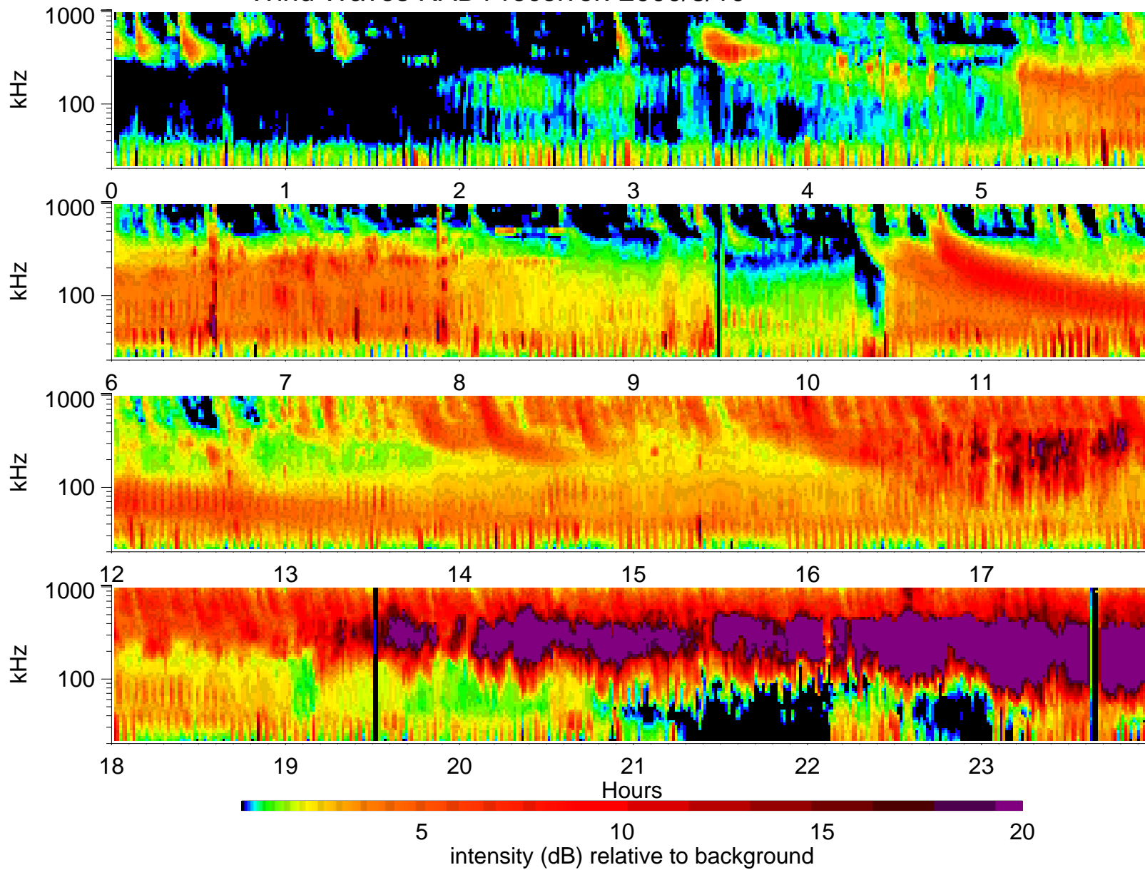
Wind Waves RAD1 receiver: 2000/8/10
