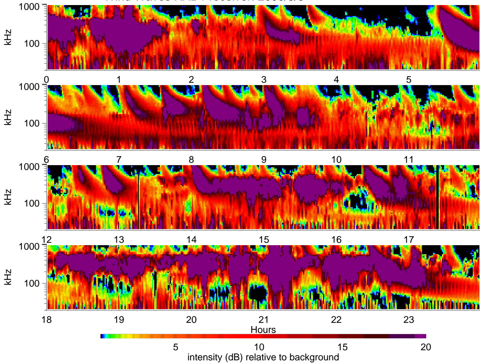
Wind Waves RAD1 receiver: 2000/8/6
