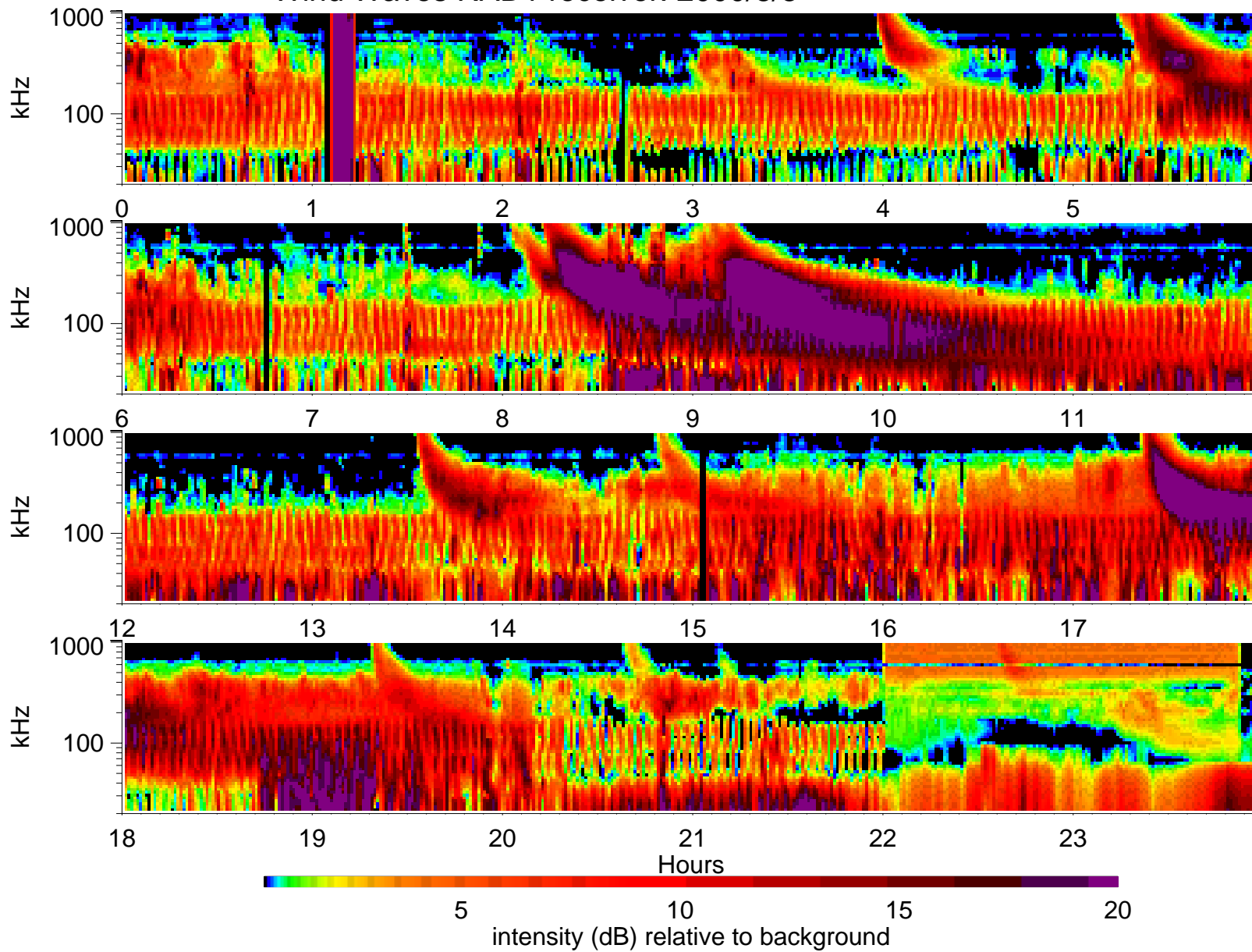
Wind Waves RAD1 receiver: 2000/8/3
