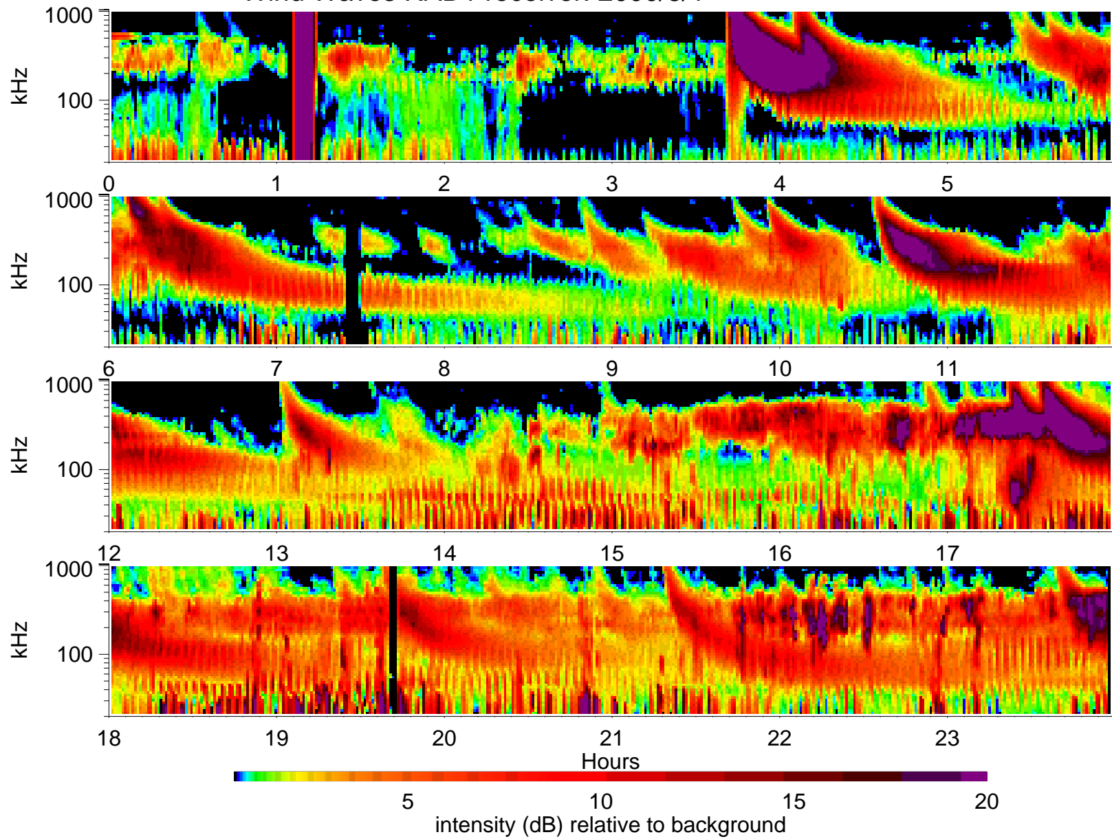
Wind Waves RAD1 receiver: 2000/8/1
