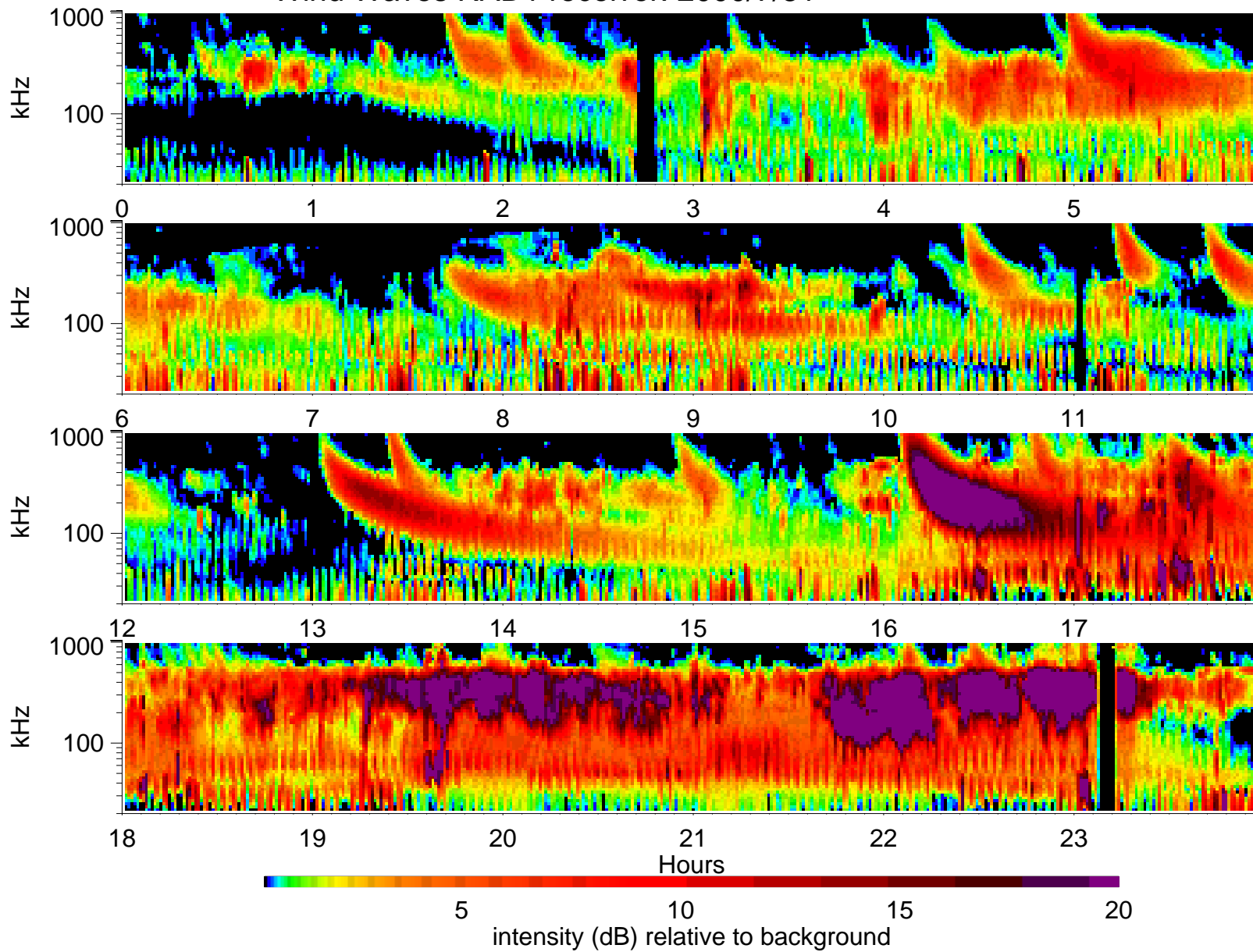
Wind Waves RAD1 receiver: 2000/7/31
