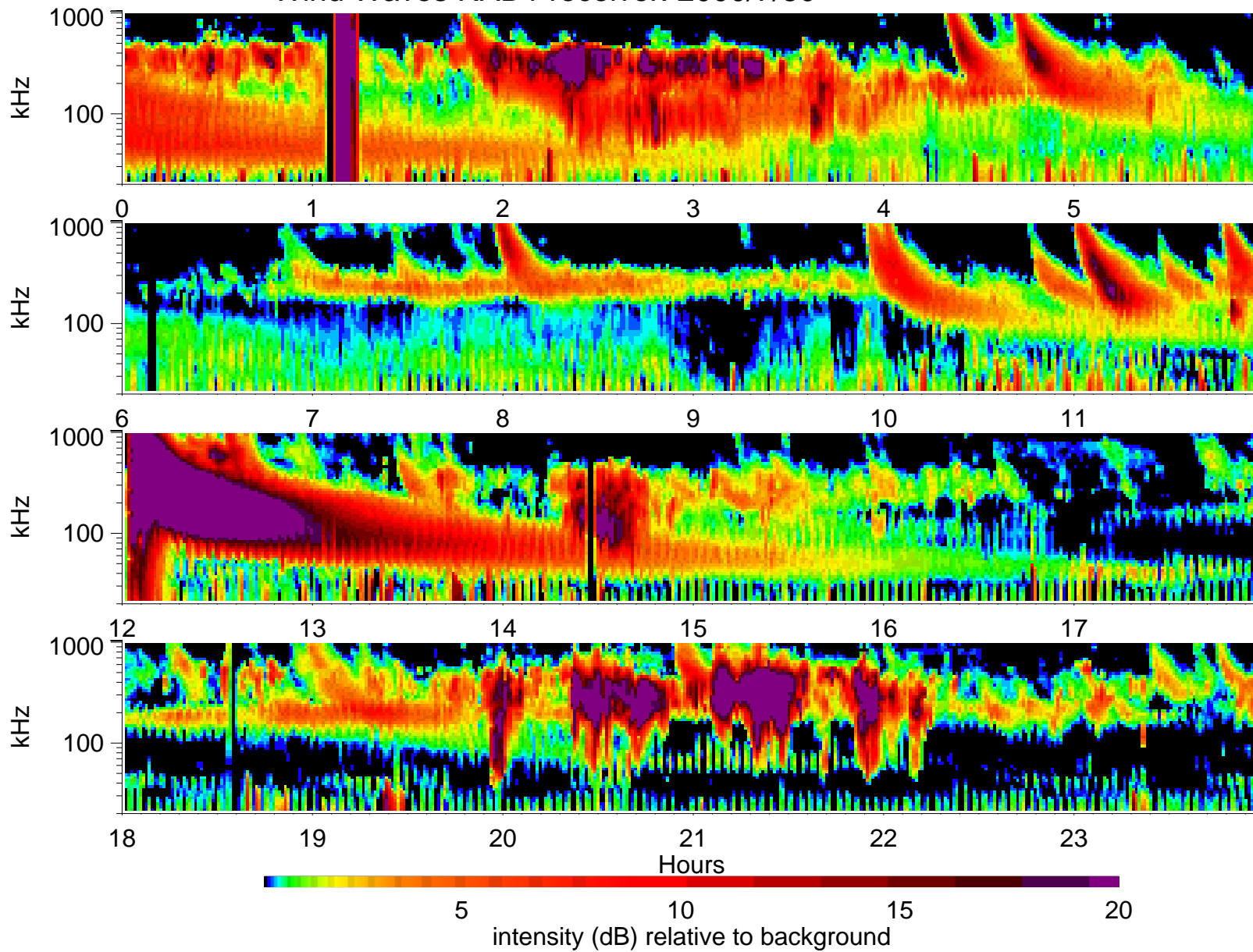
Wind Waves RAD1 receiver: 2000/7/30
