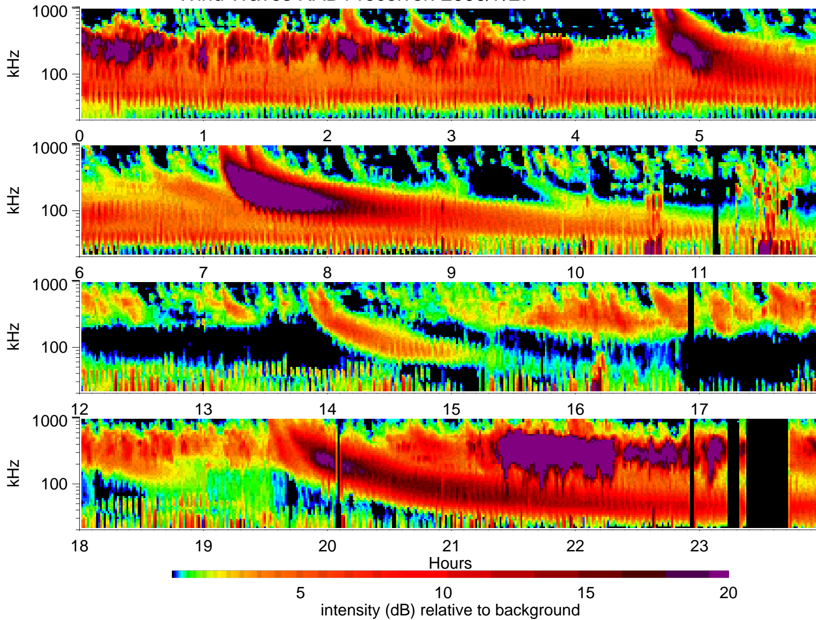
Wind Waves RAD1 receiver: 2000/7/27
