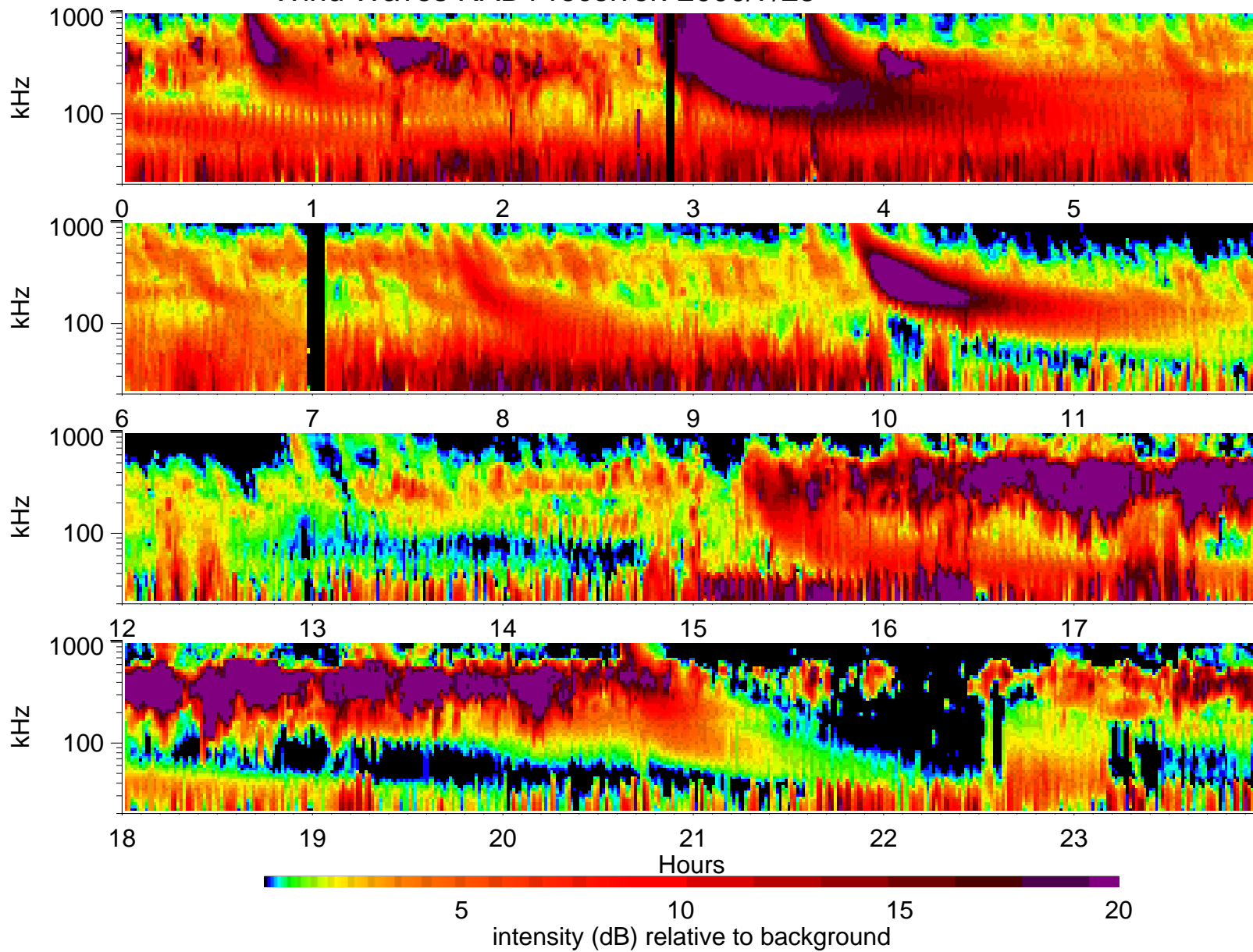
Wind Waves RAD1 receiver: 2000/7/25
