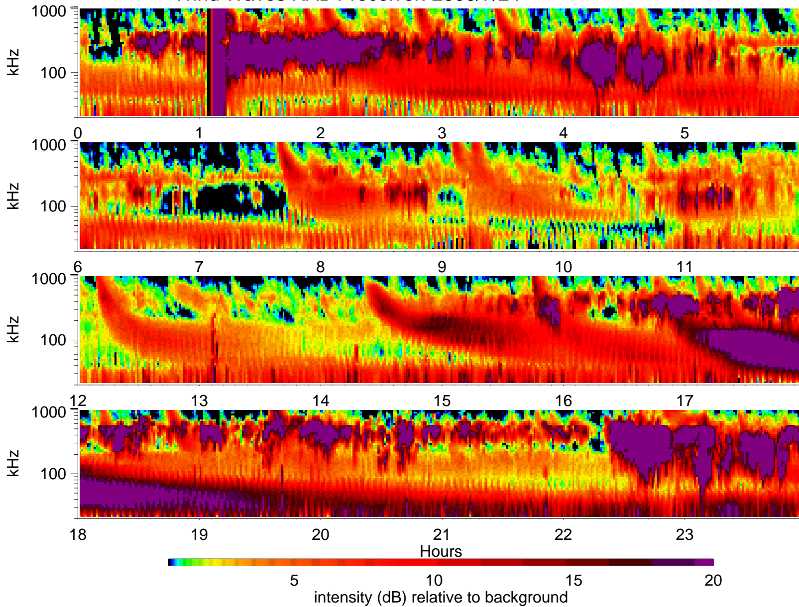
Wind Waves RAD1 receiver: 2000/7/24
