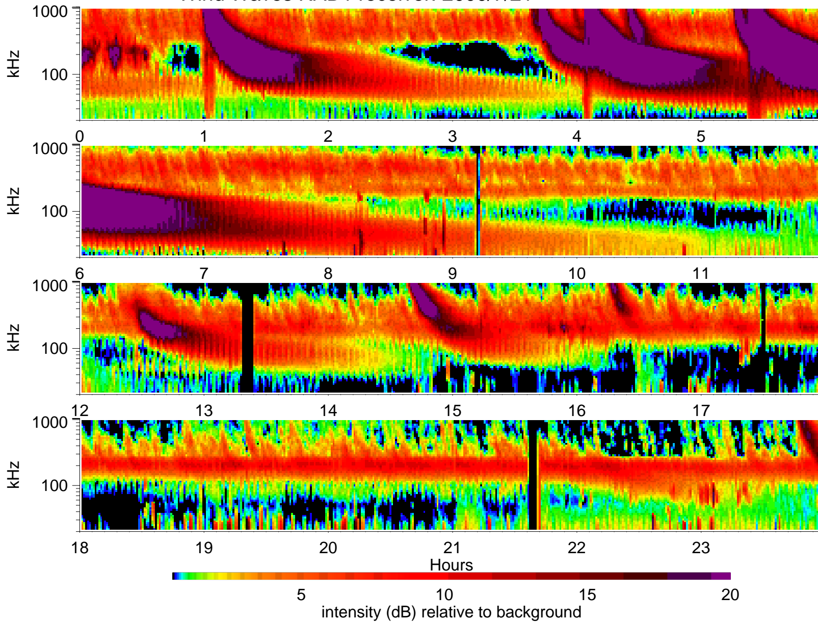
Wind Waves RAD1 receiver: 2000/7/21
